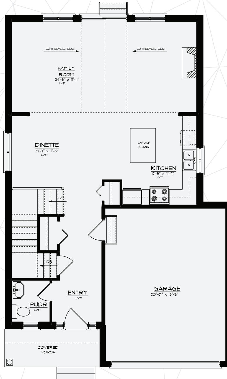
Main Floor 865 Sq. Ft.
